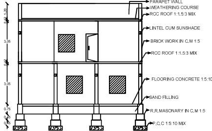
SECTION ON ABCD
