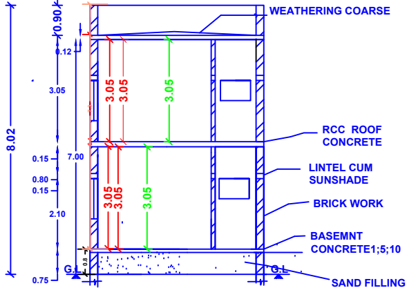
SECTION AB
