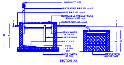
SECTION XX
