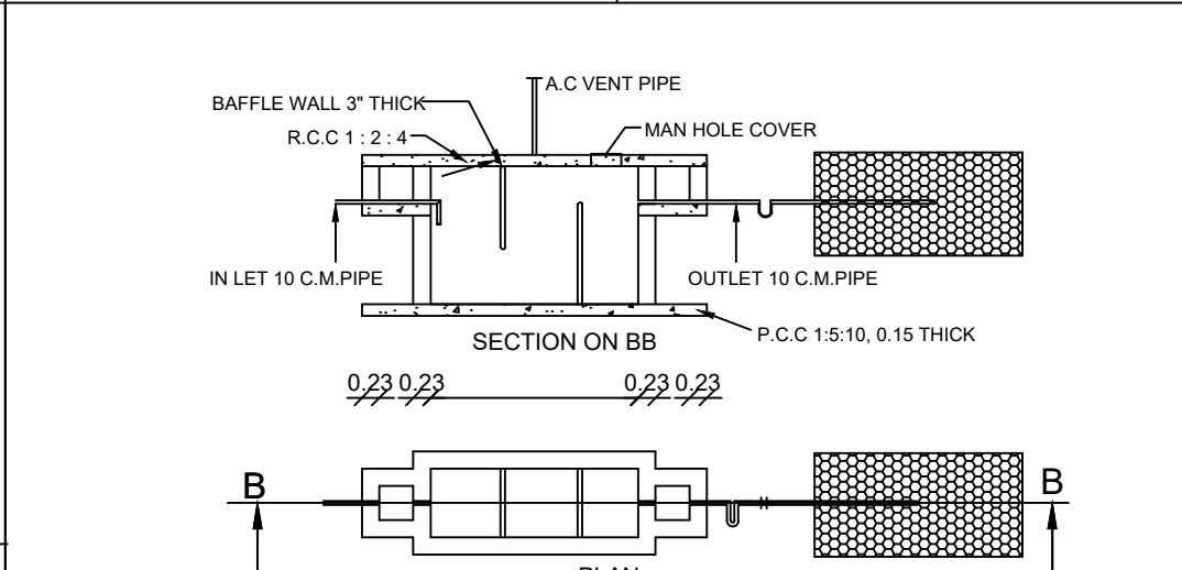
SEPTIC TANK AND TRENCH & U TRAP ADOPTED
