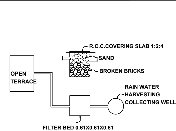
DETAILS OF RAIN WATER HARVESTING SYSTEM
