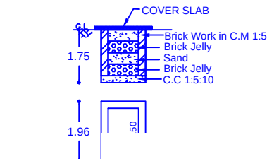
PLAN & SECTI
