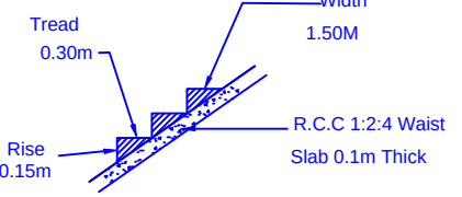
STAIRCASE DETAILS
