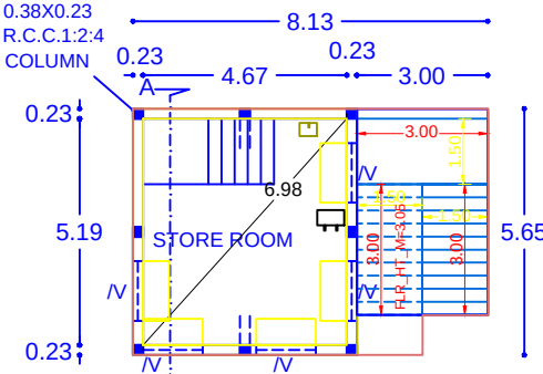
BASEMENT FLOOR PLAN
