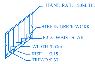
STAIR DETAIL
