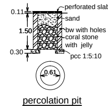
percolation pit
