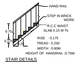
STAIR DETAILS
