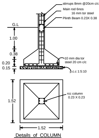
Details of COLUMN
