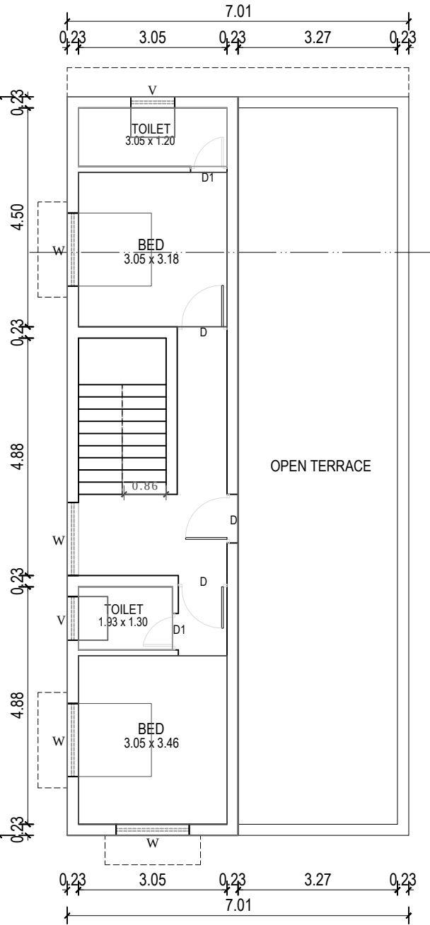
PRO.FF PLAN
