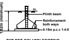
TYP.DET.COLUMN FOOTING
