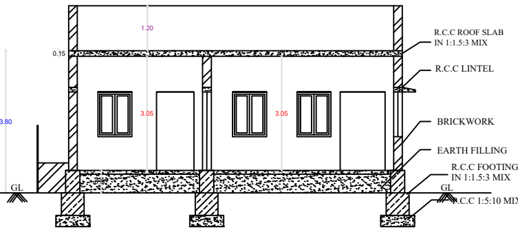
SECTION ON AA & BB
