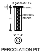
PERCOLATION PIT
