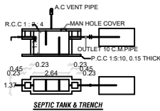
SEPTIC TANK & TRENCH
