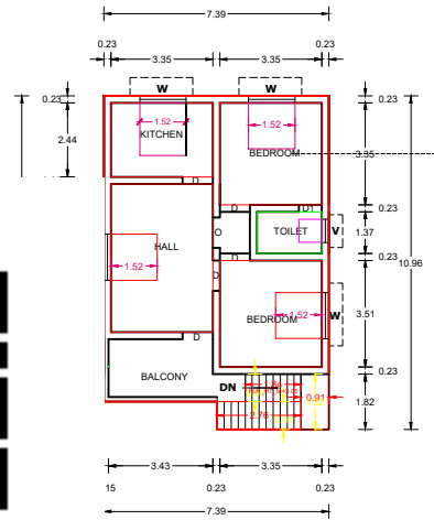
PRO.FIRST FLOOR PLAN
