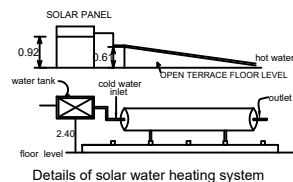
Details of solar water heating system
