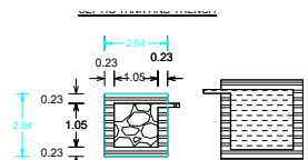
DETAILS OF FILTER BED & WELL
