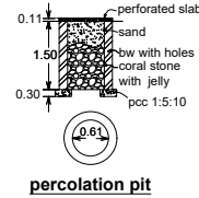
percolation pit
