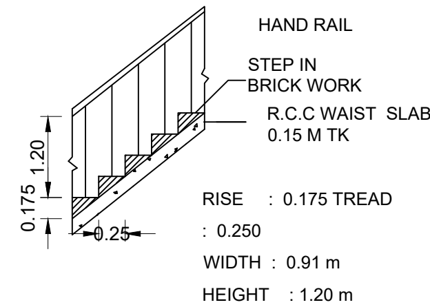
STAIR DETAILS
