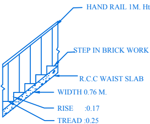
STAIR DETAIL
