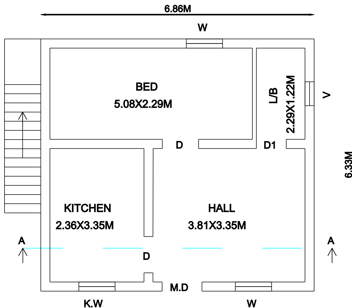
PLAN
