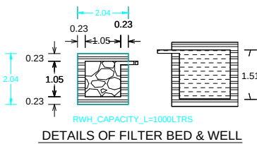
DETAILS OF FILTER BED & WELL
