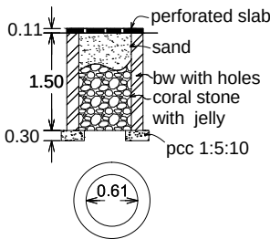
percolation pit
