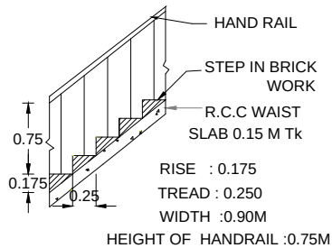
STAIR DETAILS
