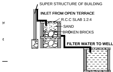
RAINWATER HARVESTING
