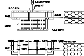
DETAILS OF FILTER BED & WELL
