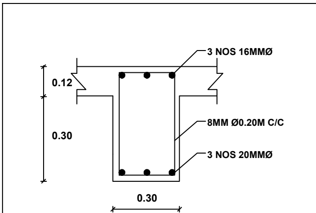
ROOF BEAM DETAILS
