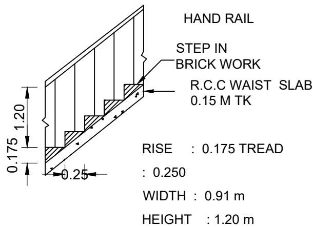
STAIR DETAILS
