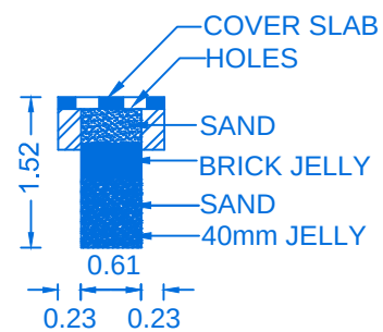
SECTION OF RAIN WATER COLLECTION TANK
