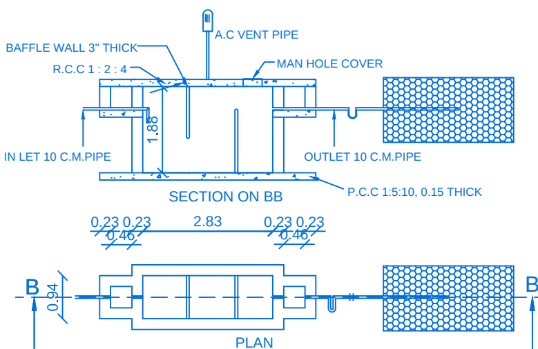
SEPTIC TANK AND TRENCH & U TRAP ADOPTED
