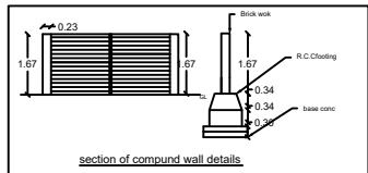
section of compound wall details
