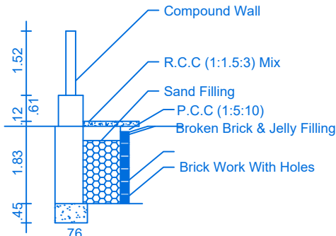
RAIN WATER HARVEST DETAILS
