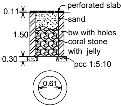
percolation pit
