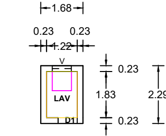
P L A N OF LAV BLOCK
