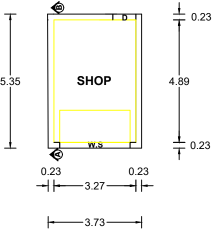
P L A N (WEST FACING SHOP)
