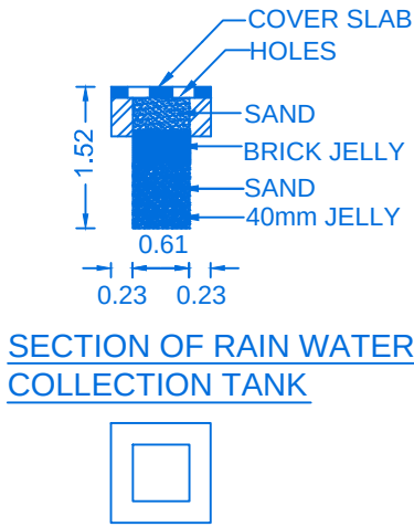
PLAN
