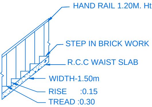
STAIR DETAIL
