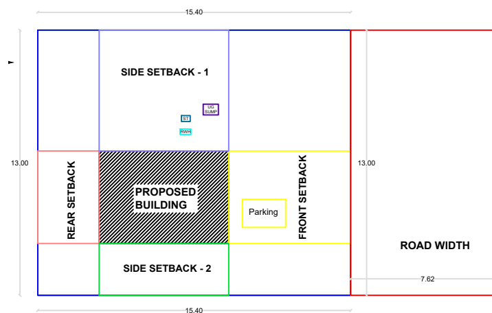
RESIDUARY PLOT SKETCH, SUPER IMPOSED SKETCH (SITE PLAN)
