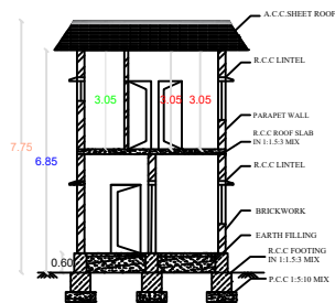
SECTION ON AA & BB
