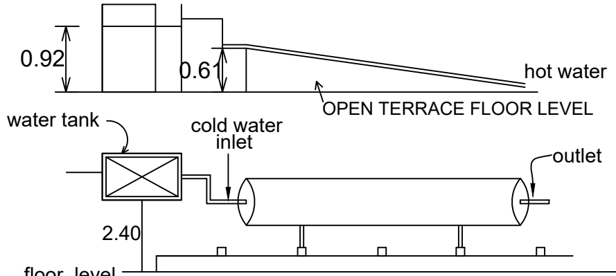
DETAILS OF SOLAR WATER HEATING SYSTEM
