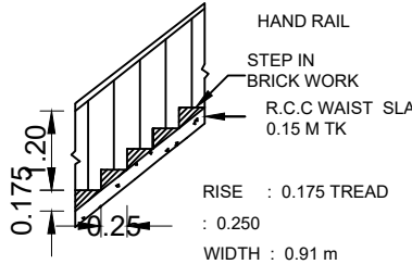
STAIR DETAILS
