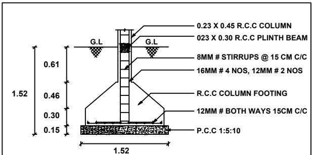
COLUMN FOOTING DETAILS
