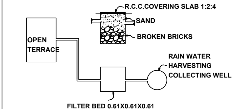
DETAILS OF RAIN WATER HARVESTING SYSTEM
