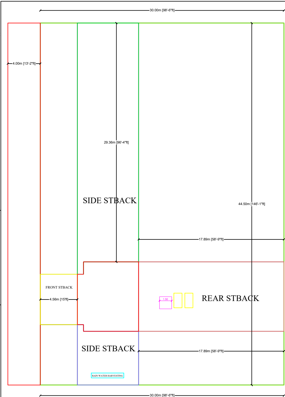
SITE SCALE (1:100)
