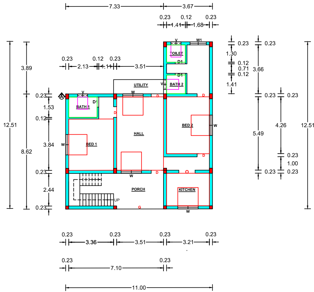
GROUND FLOOR PLAN (SOUTH FACING HOUSE)
