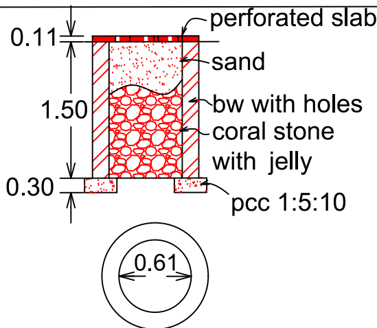
percolation pit
