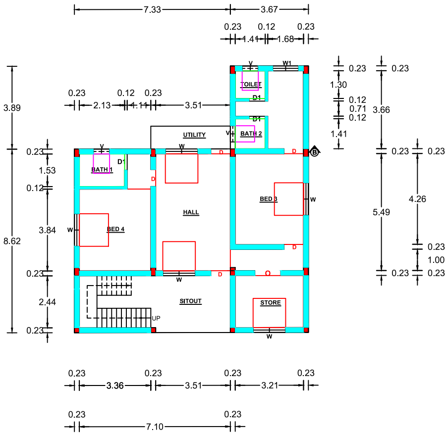
FIRST FLOOR PLAN (SOUTH FACING HOUSE)
