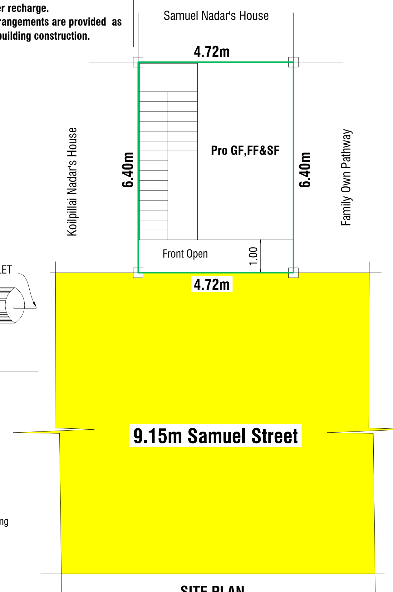
SITE PLAN
