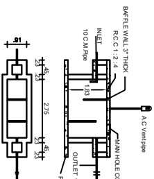
SEPTIC TANK AND TREATMENT
