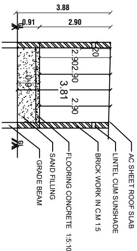
SECTION-AB
