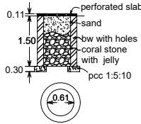
percolation pit
