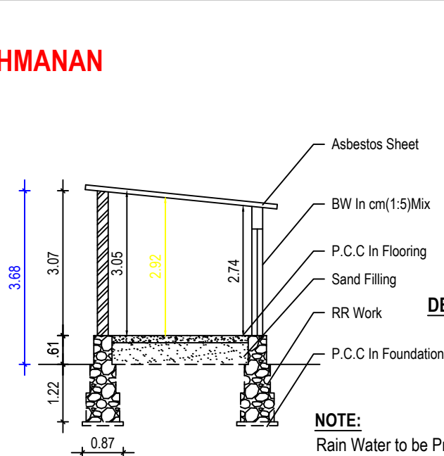
SECTION ON-AB
