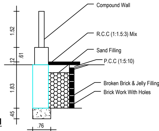
RAIN WATER HARVEST DETAILS
