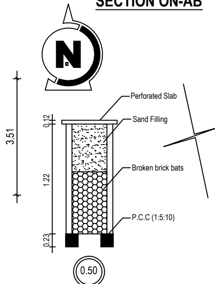
RAIN WATER COLLECTION WELL
