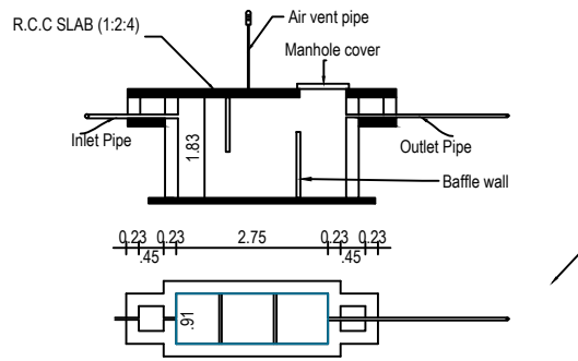
RAIN WATER COLLECTION WELL
