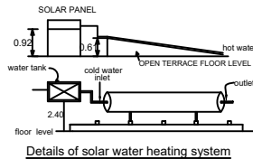
Details of solar water heating system
