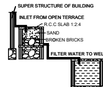
RAINWATER HARVESTING
