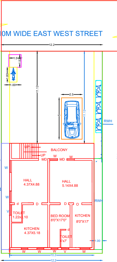
SITE PLAN SCALE 1:50
