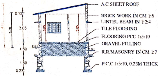
SECTION ON "V-B"
