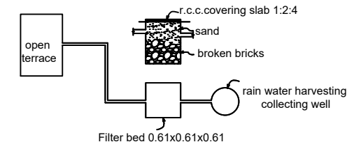
DETAILS OF RAIN WATER HARVESTING SYSTEM
