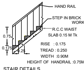
STAIR DETAILS
