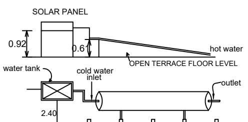
Details of solar water heating system
