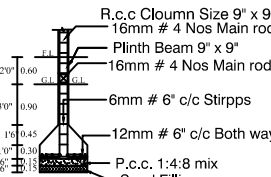
COLUMN DETIAL
