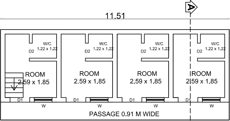
SITE PLAN
