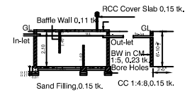
SEPTIC TANK & SOAK PIT
