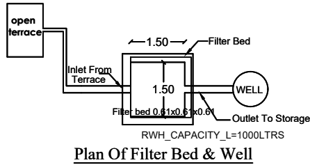
Plan Of Filter Bed & Well
