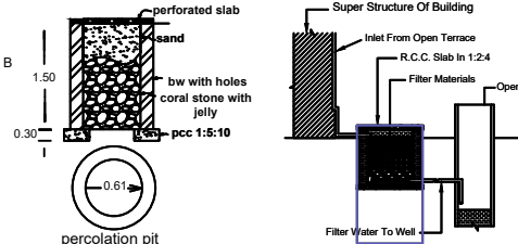
Details Of Rainwater Harvesting System
