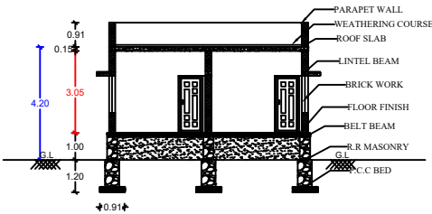
CROSS SECTION VIEW AB
