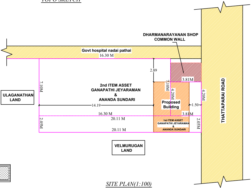
SITE PLAN(1:100)
