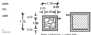
DETAILS OF FILTER BED & WELL
