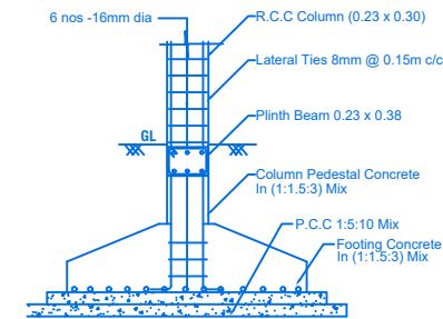
COLUMN FOOTING DETAILS
