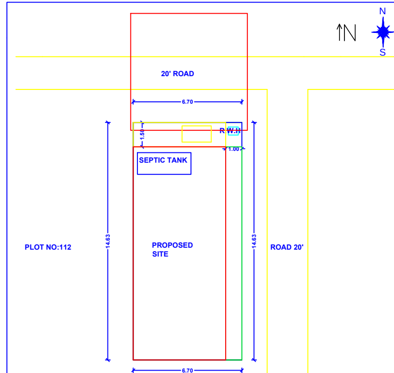
SITE PLAN
