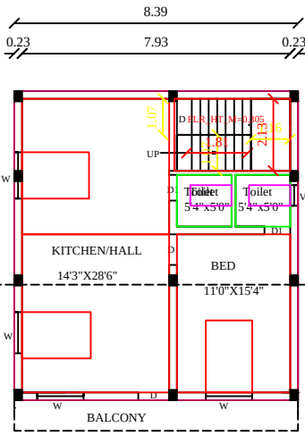
F.FLOOR PLAN
