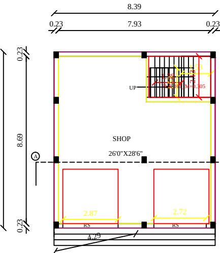
G.FLOOR PLAN
