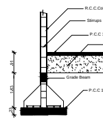
COLUMN DETAIL
