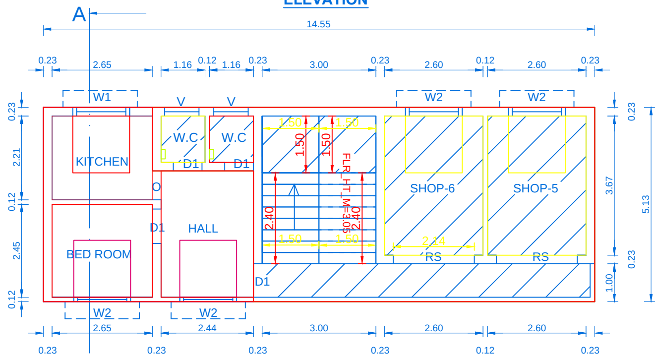
EXG & PROP.FIRST FLOOR PLAN
