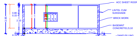
SECTION AB
