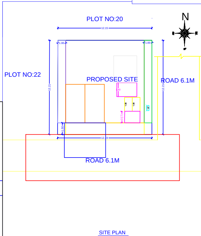
SITE PLAN
