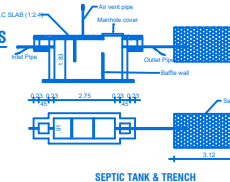
SEPTIC TANK & TRENCH
