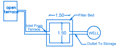
Plan Of Filter Bed & Well
