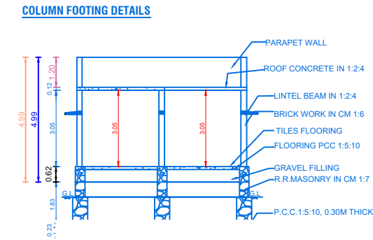
COLUMN FOOTING DETAILS
