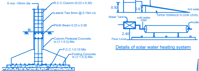
COLUMN FOOTING DETAILS
