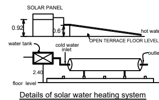
DETAILS OF SOLAR WATER HEATING SYSTEM
