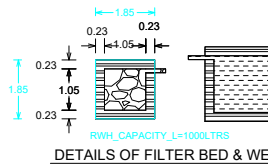
DETAILS OF FILTER BED & WELL
