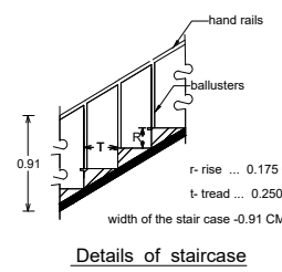
DETAILS OF STAIRCASE
