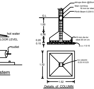
DETAILS OF COLUMN
