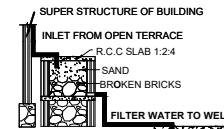
RAINWATER HARVESTING
