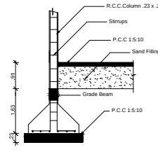
COLUMN DETAIL
