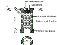
PERCOLATION PIT FOR 30 Sq. m. (Scale:- 1:50)
