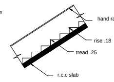
STAIR
