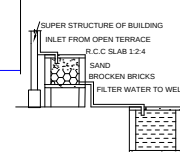
RAINWATER HARVESTING
