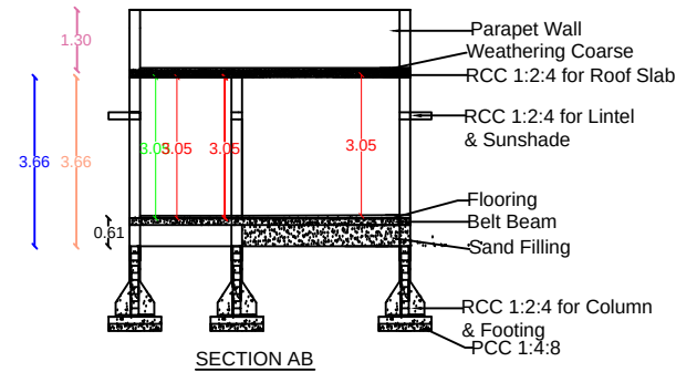
SECTION AB
