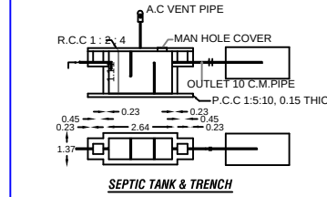
SEPTIC TANK & TRENCH
