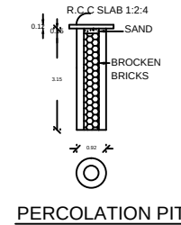
PERCOLATION PIT
