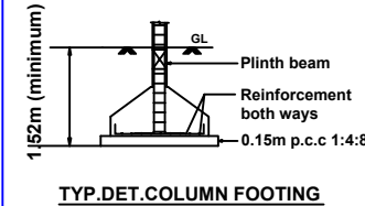
TYP.DET.COLUMN FOOTING
