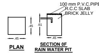
PLAN SECTION OF RAIN WATER PIT
