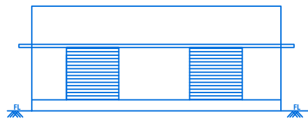
FRONT ELEVATION
