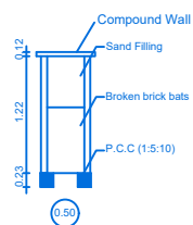
RAIN WATER COLLECTION WELL
