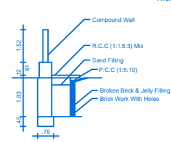
RAIN WATER HARVEST DETAILS
