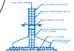
COLUMN FOOTING DETAILS
