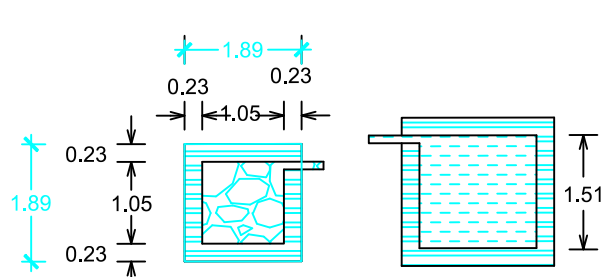
RWH_CAPACITY_L=1000LTRS DETAILS OF FILTER BED & WELL
