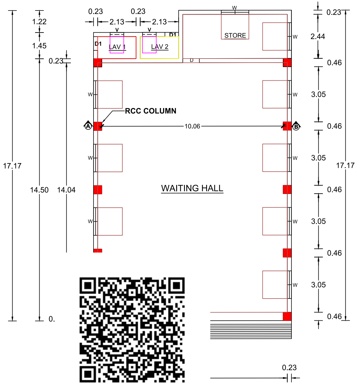
P L A N (SOUTH FACING WAITING HALL)
