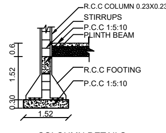
COLOUMN DETAILS
