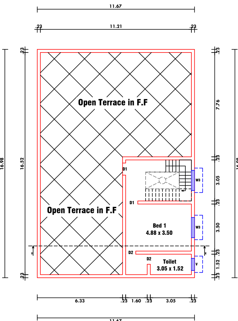
PRO. FIRST FLOOR
