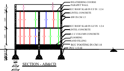
SECTION - AB&CD
