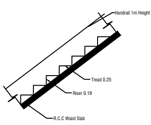
STAIR DETAILS
