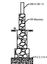
DETAILS OF RR MASONARY
