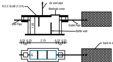
SEPTIC TANK & TRENCH
