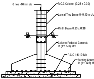
COLUMN FOOTING DETAILS
