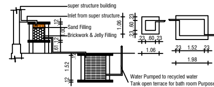
DETAIL PLAN FOR FILTER MEDIA & SUMP
